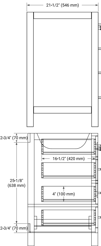
SIDE VIEW
