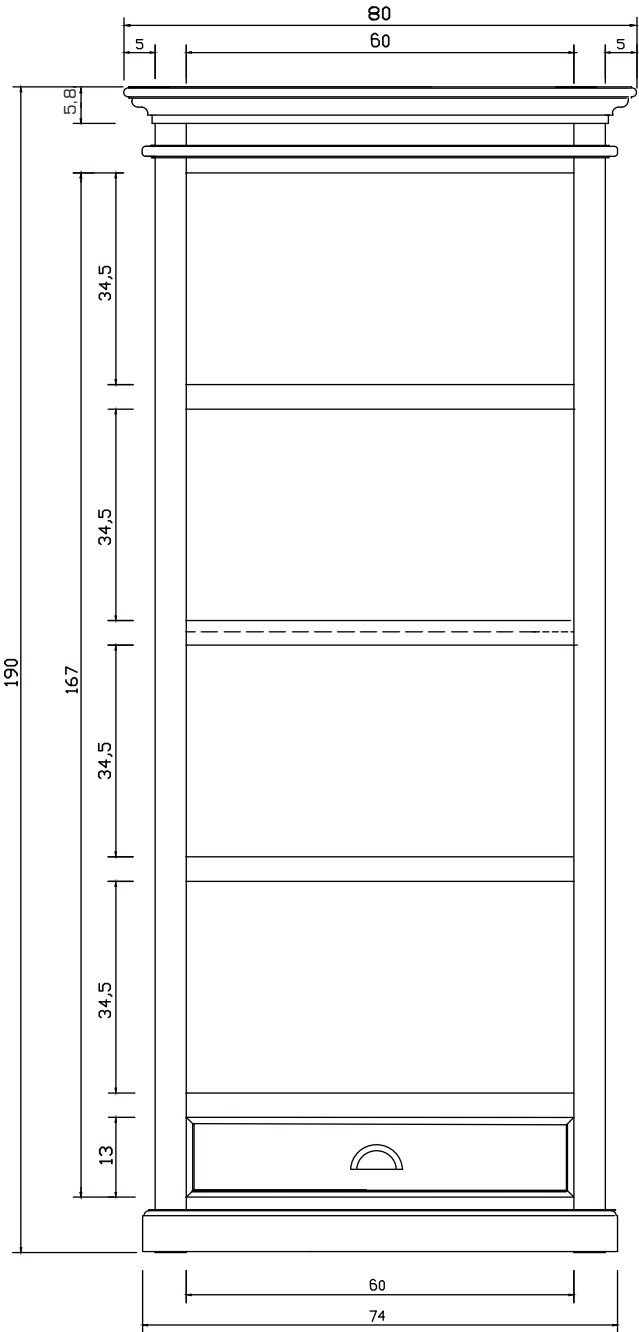
FRONT VIEW
