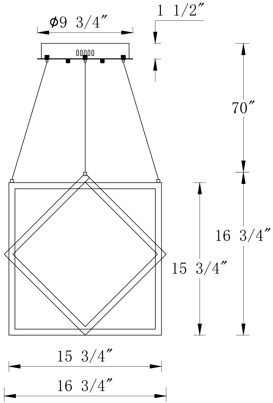
FRONT VIEW
