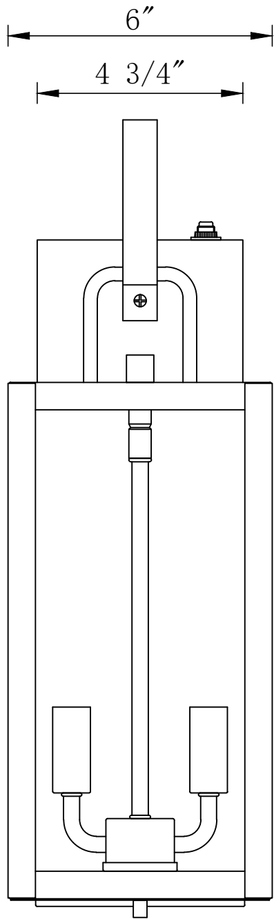
FRONT VIEW
