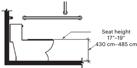
ADA Accessible Toilet Seat Height Requirements
