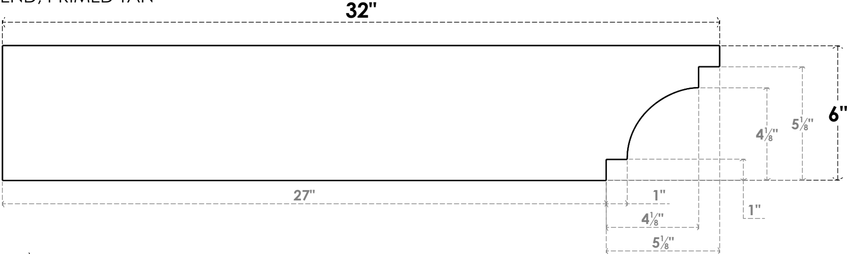
SIDE PROFILE
