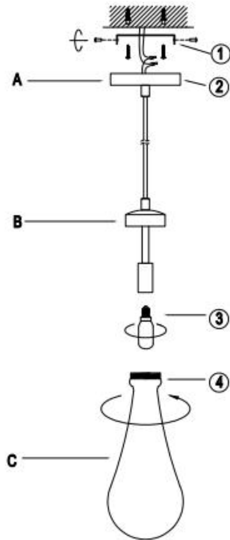
Installation sequence diagram
