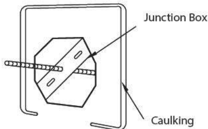
Fig.3 Sealing
