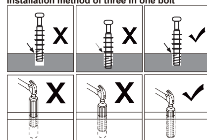
Installation method of three in one bolt
