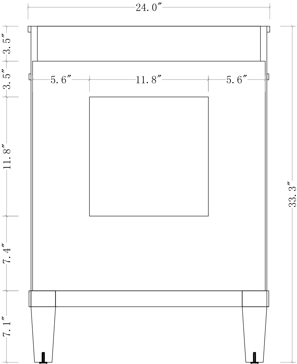
BACK VIEW
