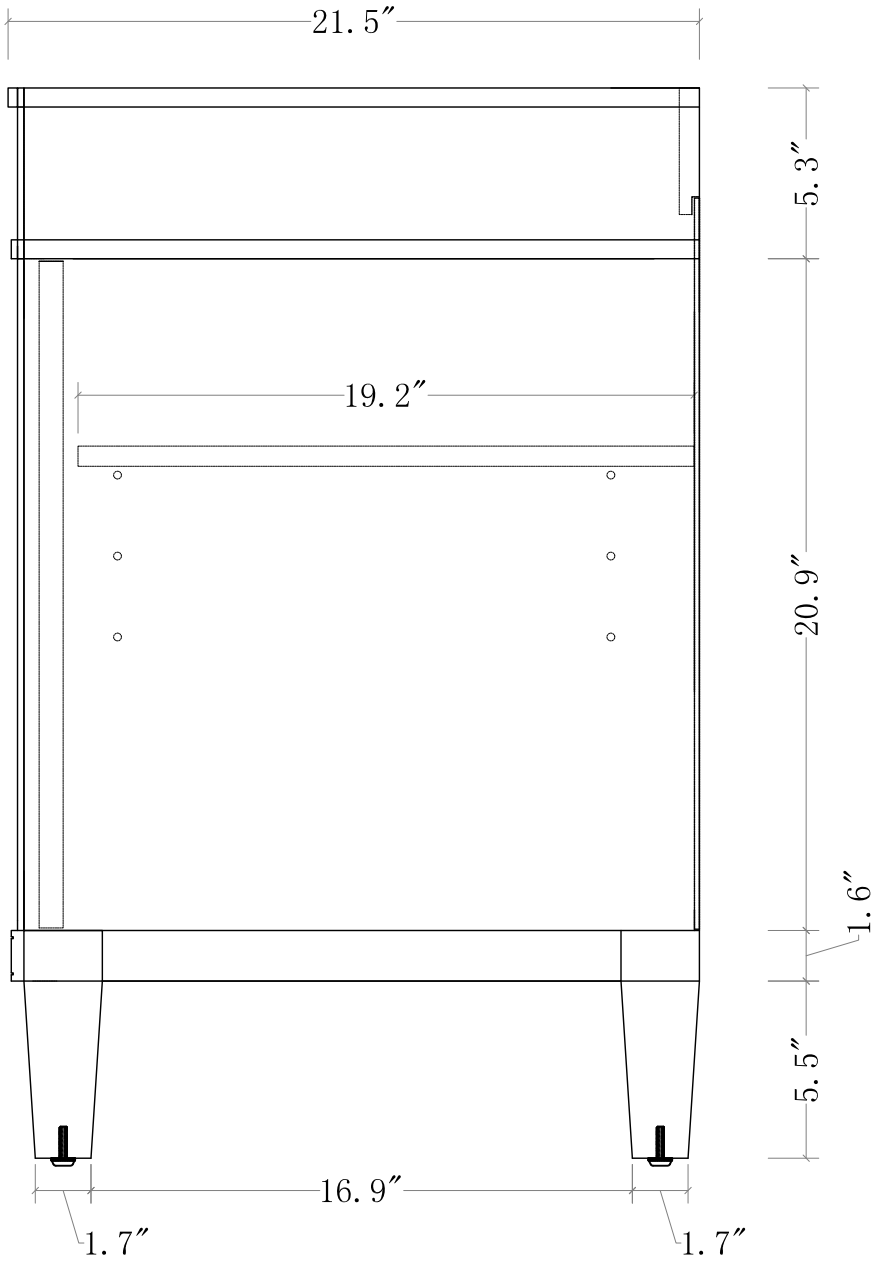
SIDE VIEW
