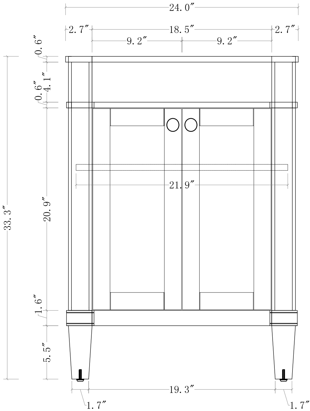
FRONT VIEW
