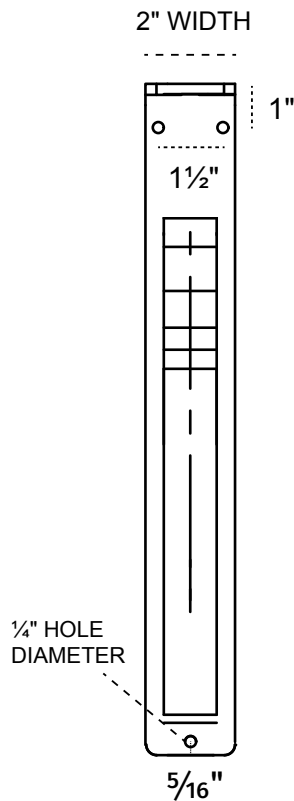
FRONT PROFILE
