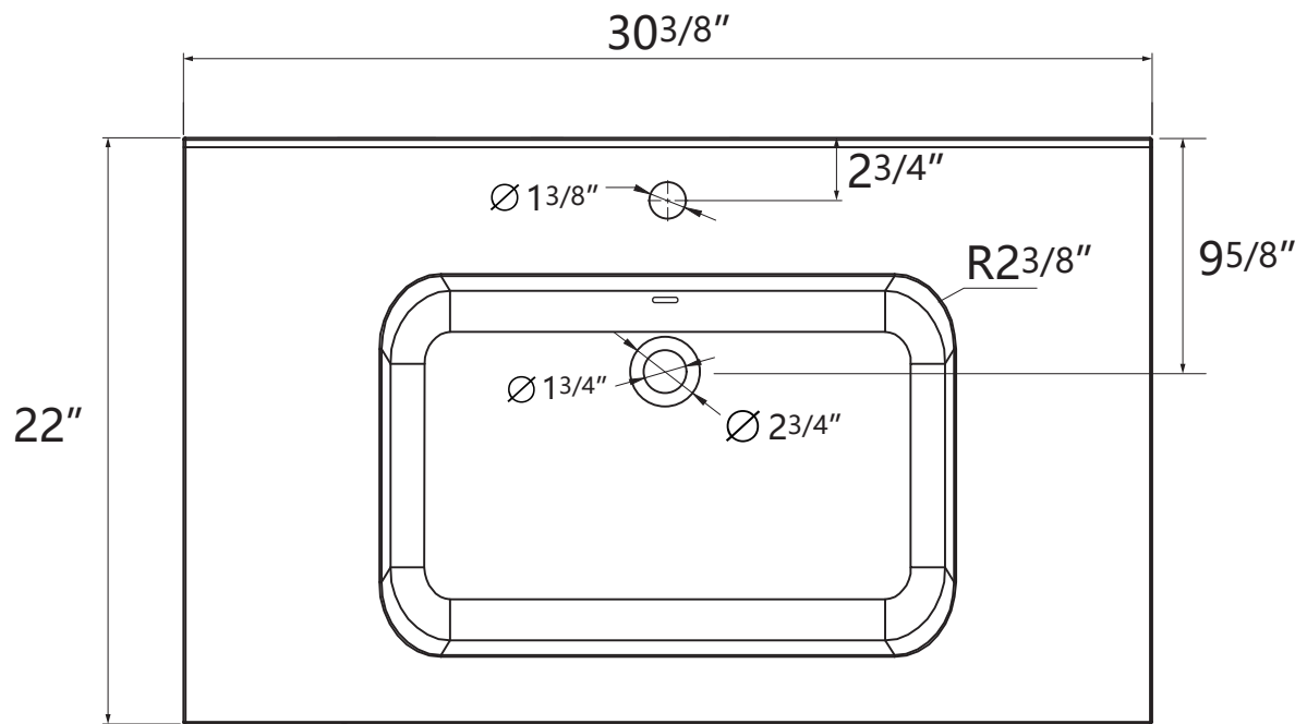
Top View
