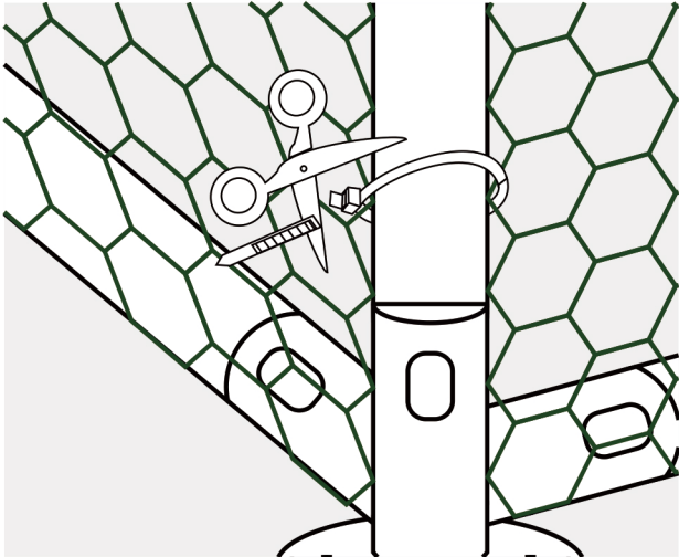
Cut the excess off the cable ties
