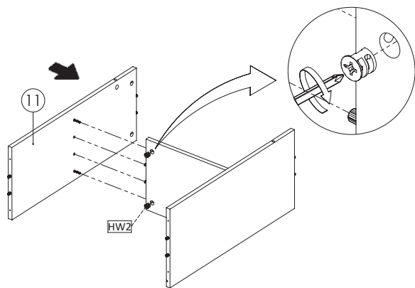
STEP11: Insert Storage Center Panel (11). Secure with Camlock (HW2) And Tighten It Using Screwdriver.
