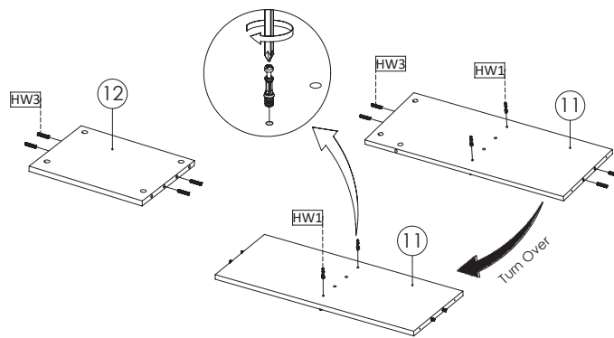
STEP10: Insert Cambolt (HW1) Into Storage Center Panel (11). Insert Wooden Dowel (HW3) Into Storage Center Panel (11) And Storage Left Fixed Shelf (12)
