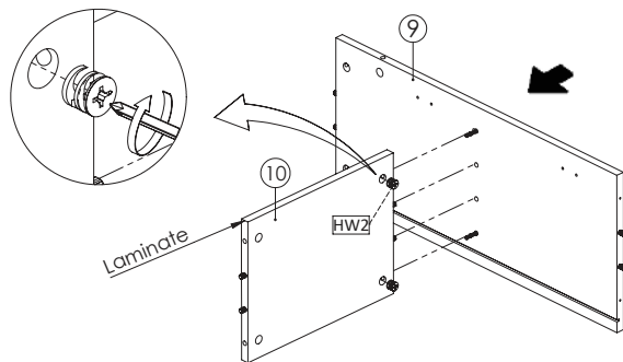
STEP9: Attach Storage Right Fixed Shelf (10) Into Storage Right Side Panel (9). Secure with Camlock (HW2) And Tighten It Using Screwdriver.
