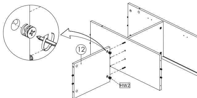
STEP12: Insert Storage Left Fixed Shelf (12). Secure with Camlock (HW2) And Tighten It Using Screwdriver.
