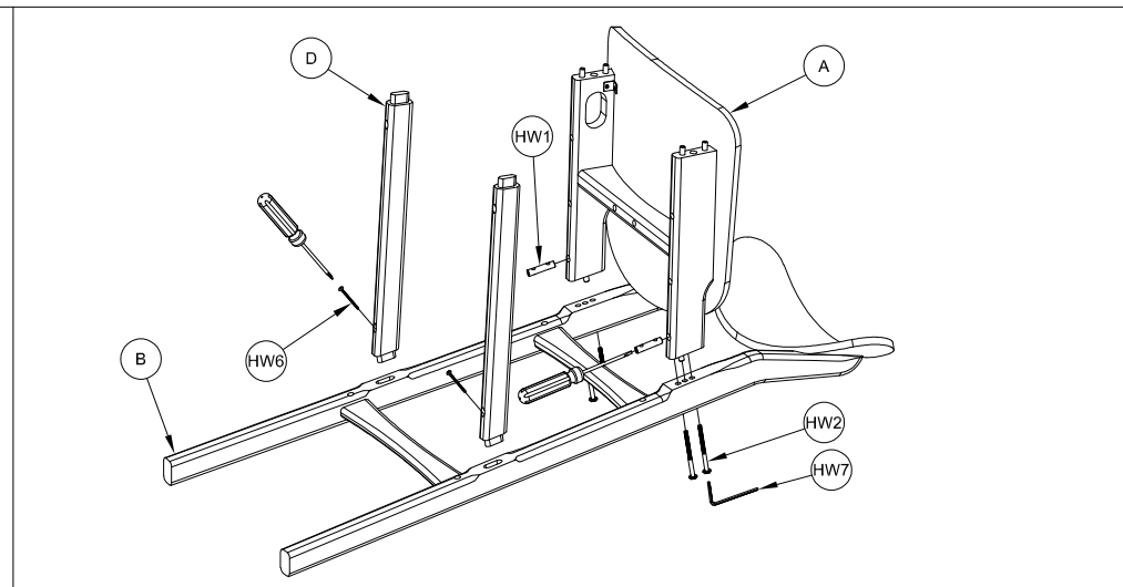
STEP 2: Assemble the seat to the back leg part. Make sure to apply all the bolt into the holes properly before tightening.
