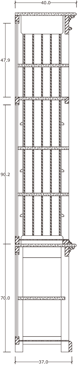
SECTION DETAIL
