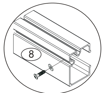
Screw mounting position
