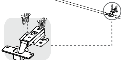
Full overlay hinge
