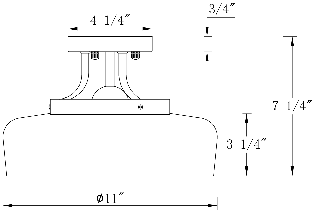
FRONT VIEW
