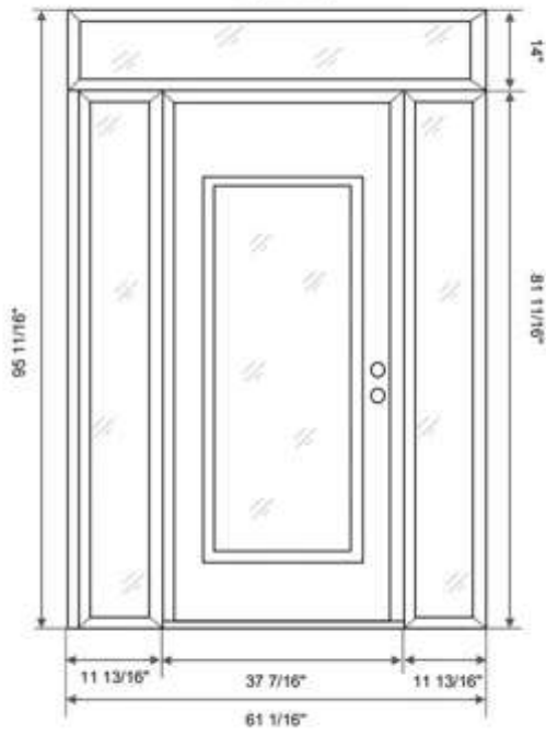
With Two Sidelites and Transom (Actual size)
