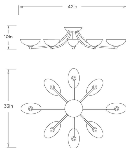
DFC29 ZAMORA FLUSH MOUNT
