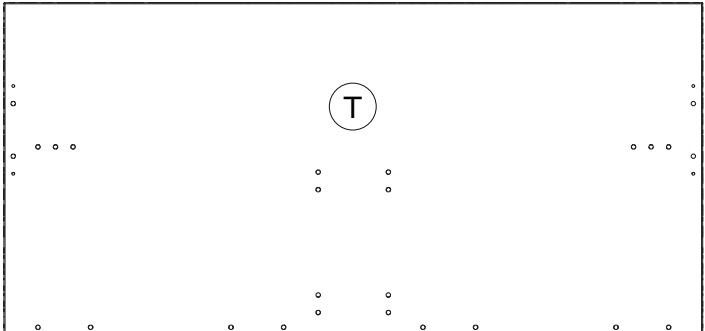
TE0608 1274x600x30mm
