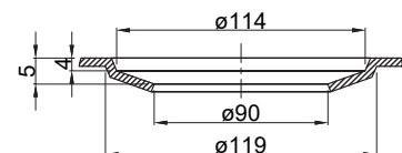
DRAIN
