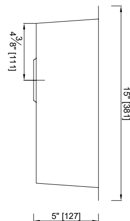
SIDE
