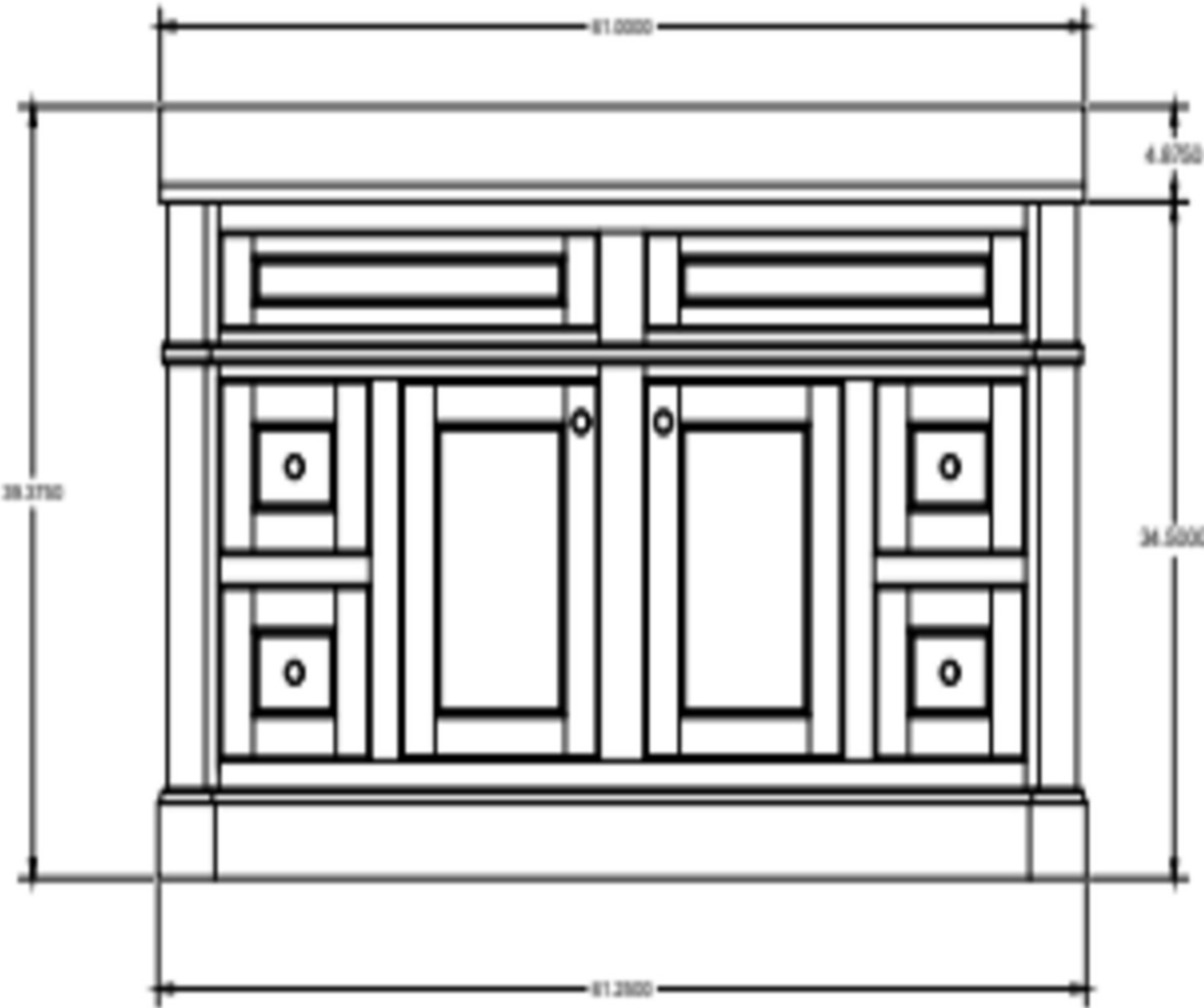
FRONT VIEW
