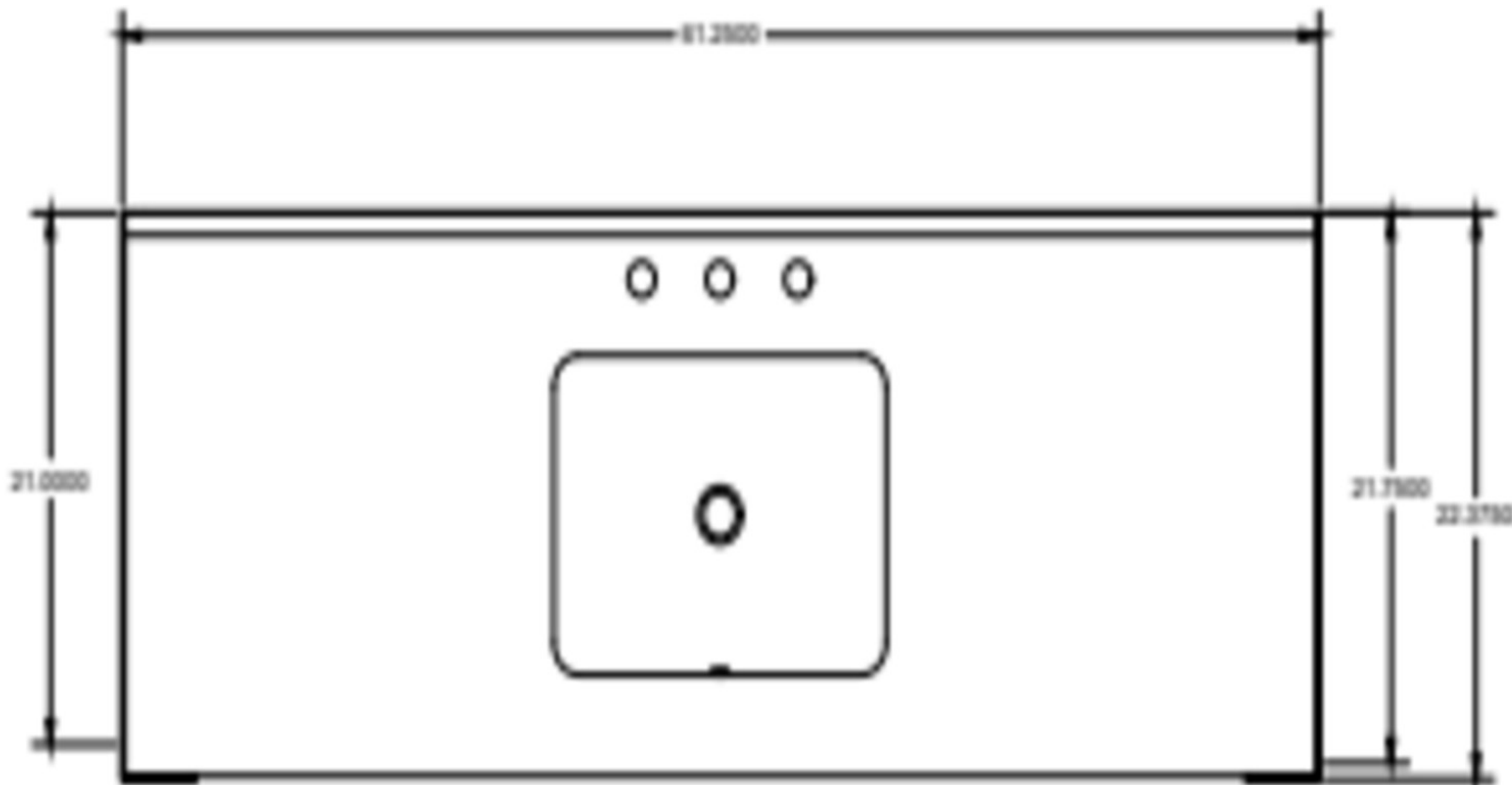
TOP VIEW
