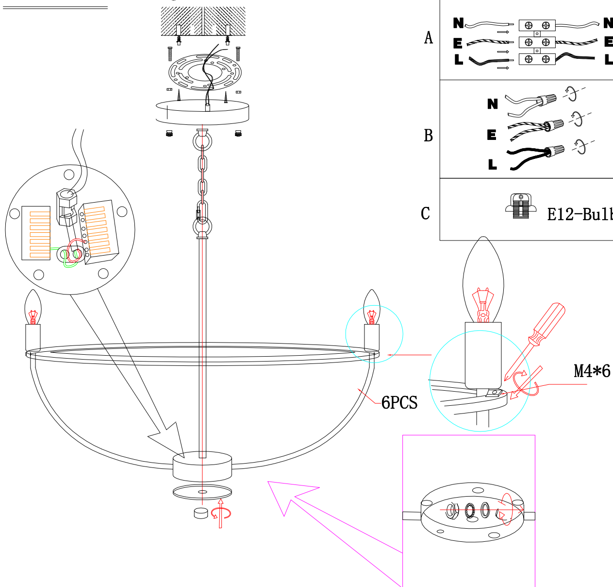
Wiring diagram
