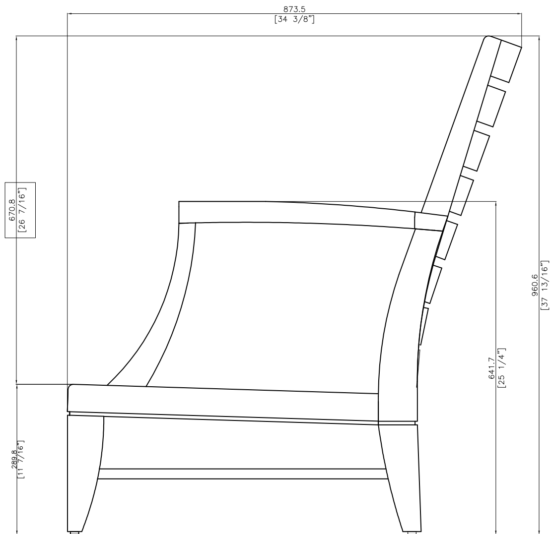
SIDE VIEW
