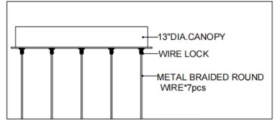
CANOPY DETAIL
