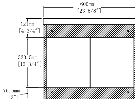
Back View
