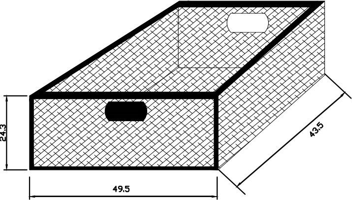
DETAIL BASKET
