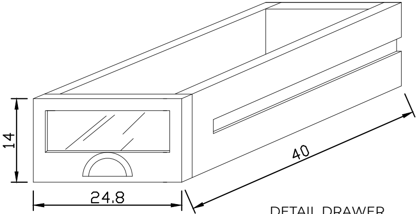
DETAIL DRAWER
