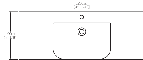
Top View(48S)
