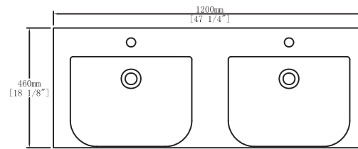
Top View(48D)
