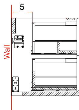
Side view for plumbing
