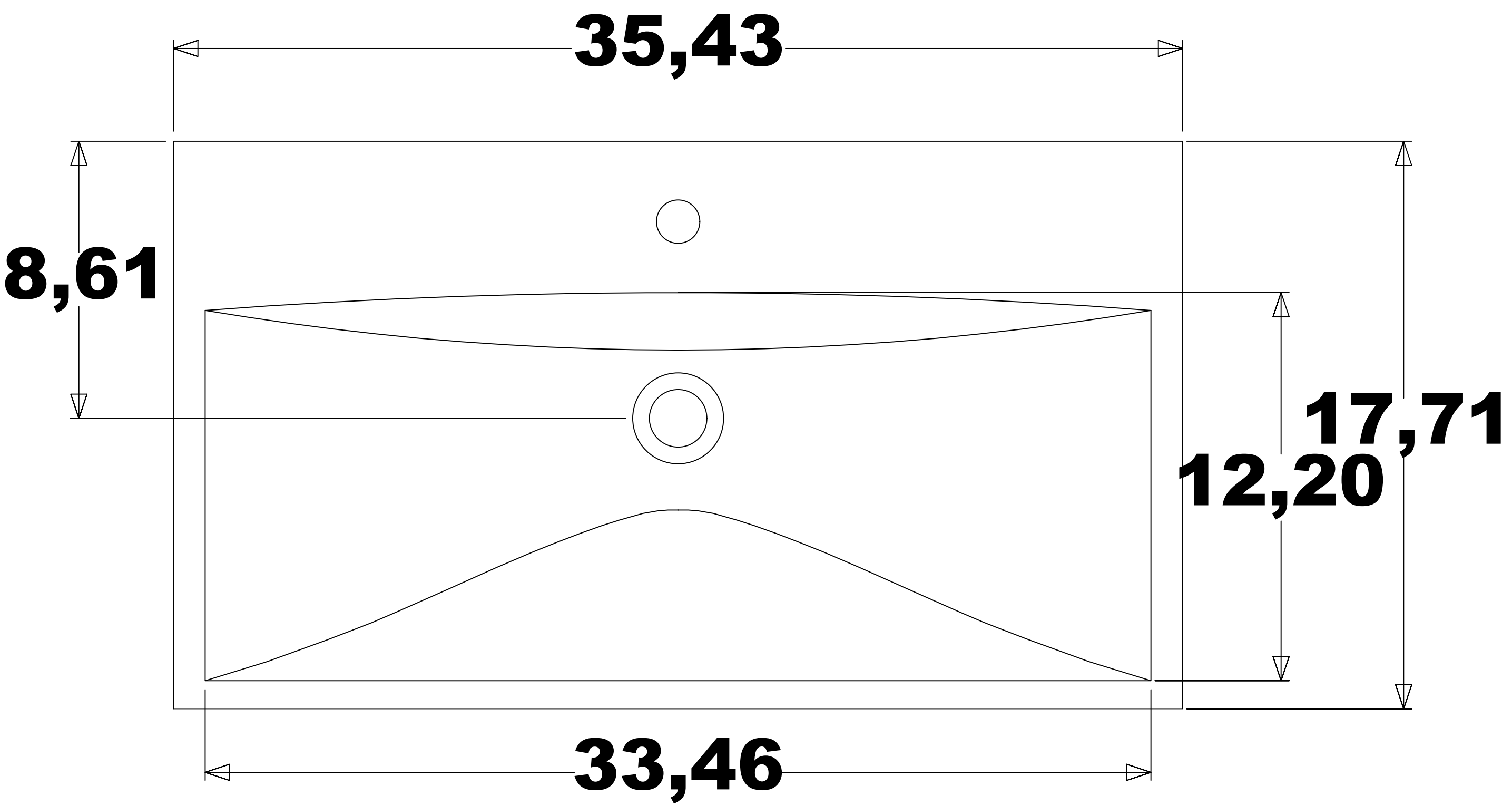
TOP VIEW
