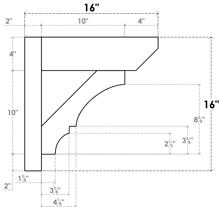
SIDE PROFILE
