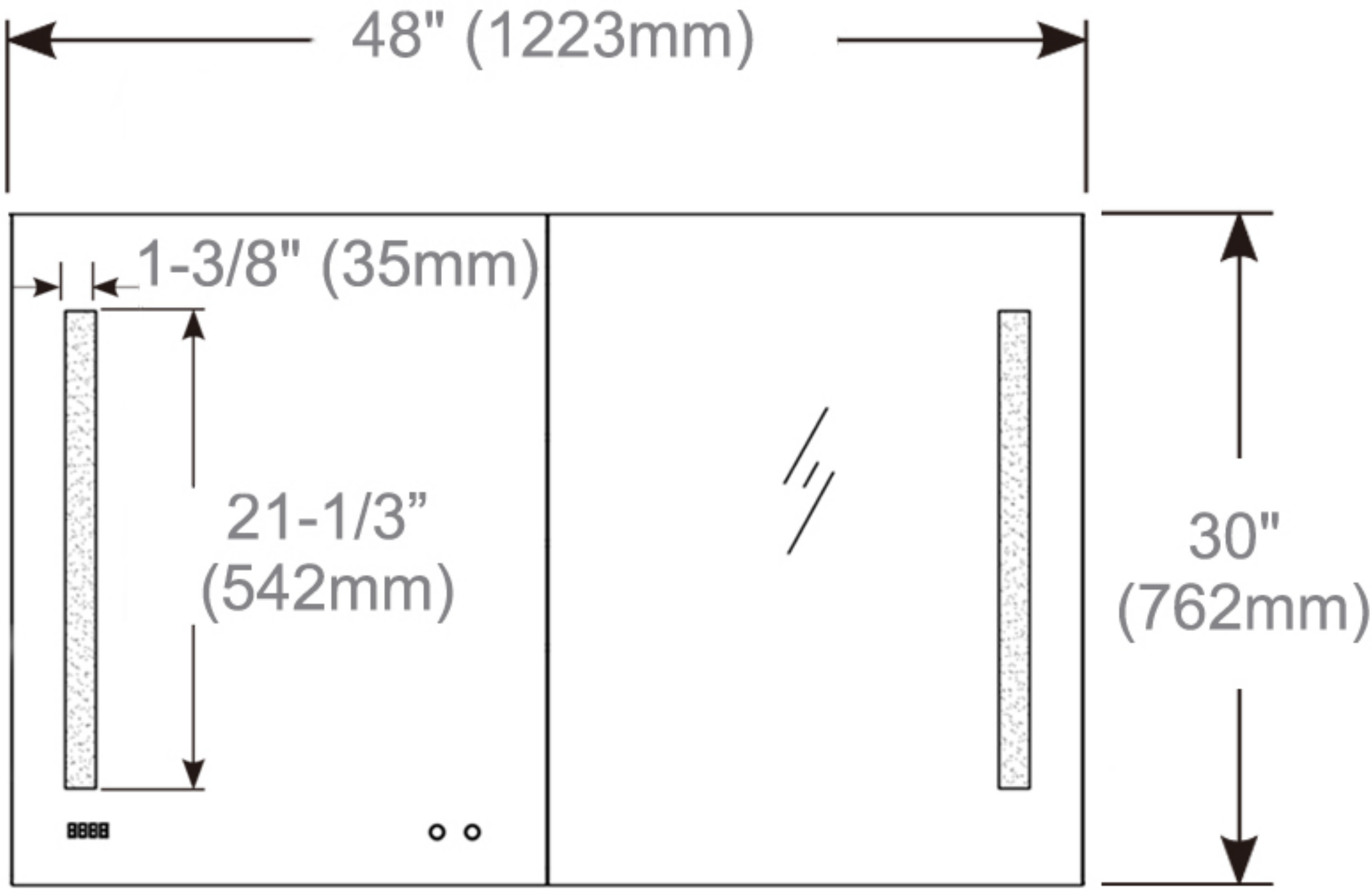
Cabinet Dimensions
