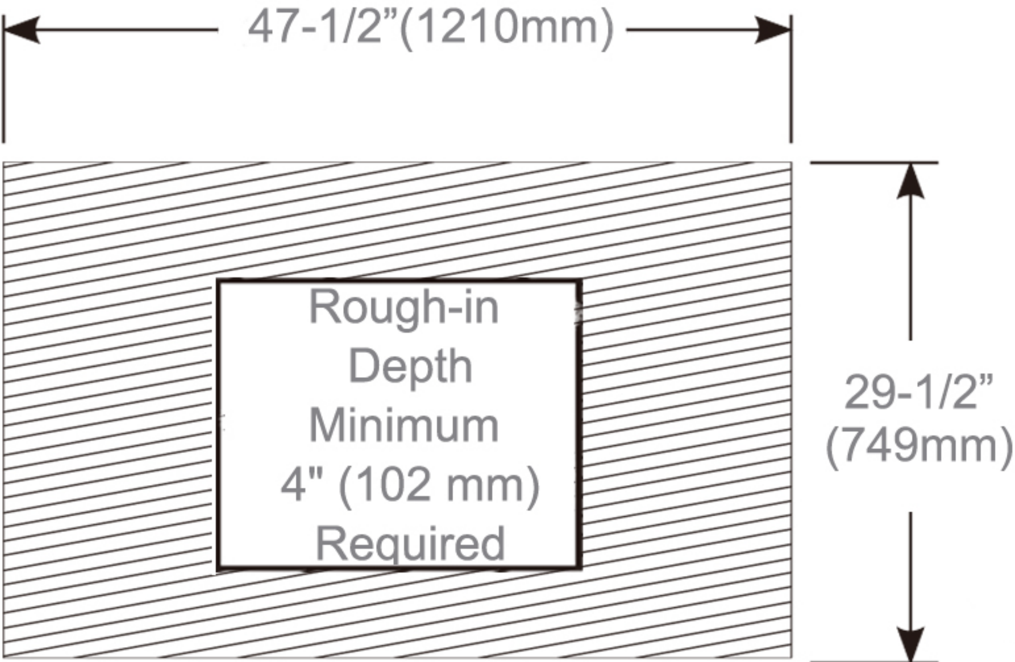
Rough-in Dimensions
