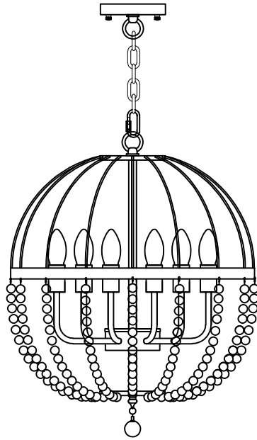
6x Max 60W Candelabra Base
