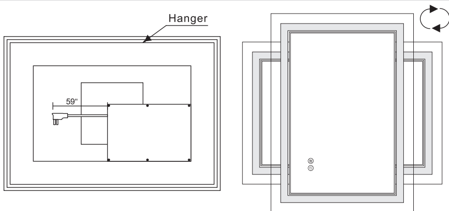
Horizontal/ Vertical Installation
