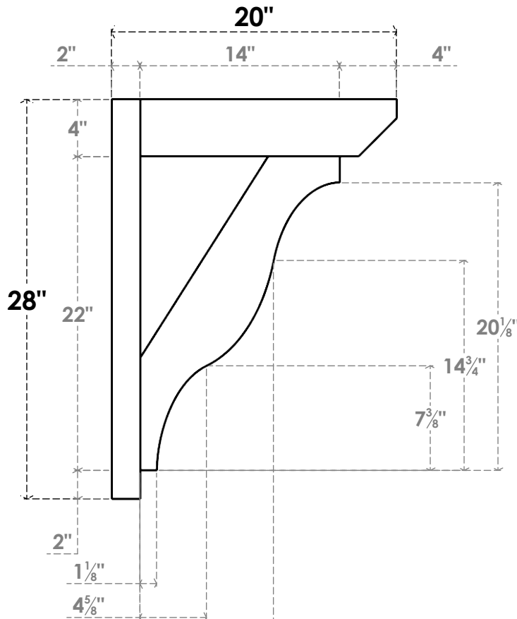
SIDE PROFILE
