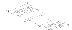
Handle's Dimension
