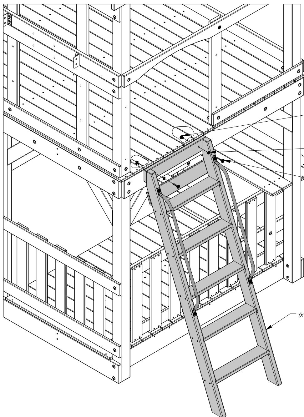
379 (x2) T-NUT - 5/16"
