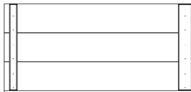
RP5 | RIGHT PORCH ROOF PANEL - W2A02654 (1) 1 5/8"x15 5/8"x32 7/8" (42x396x834)
