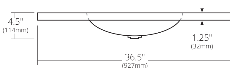
SIDE VIEW
