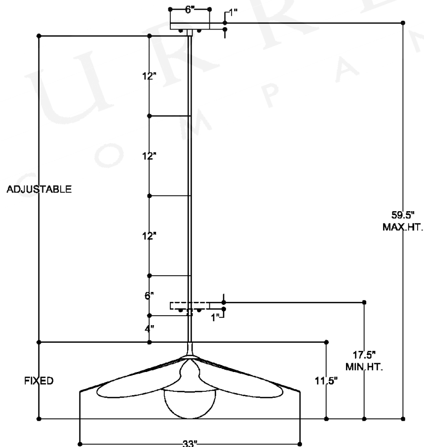
FRONT VIEW
