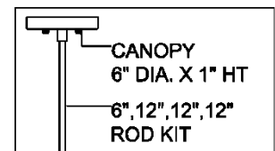
CANOPY DETAIL
