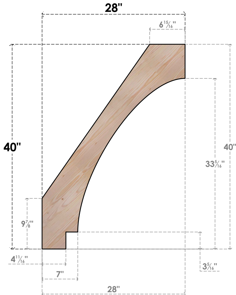
SIDE
