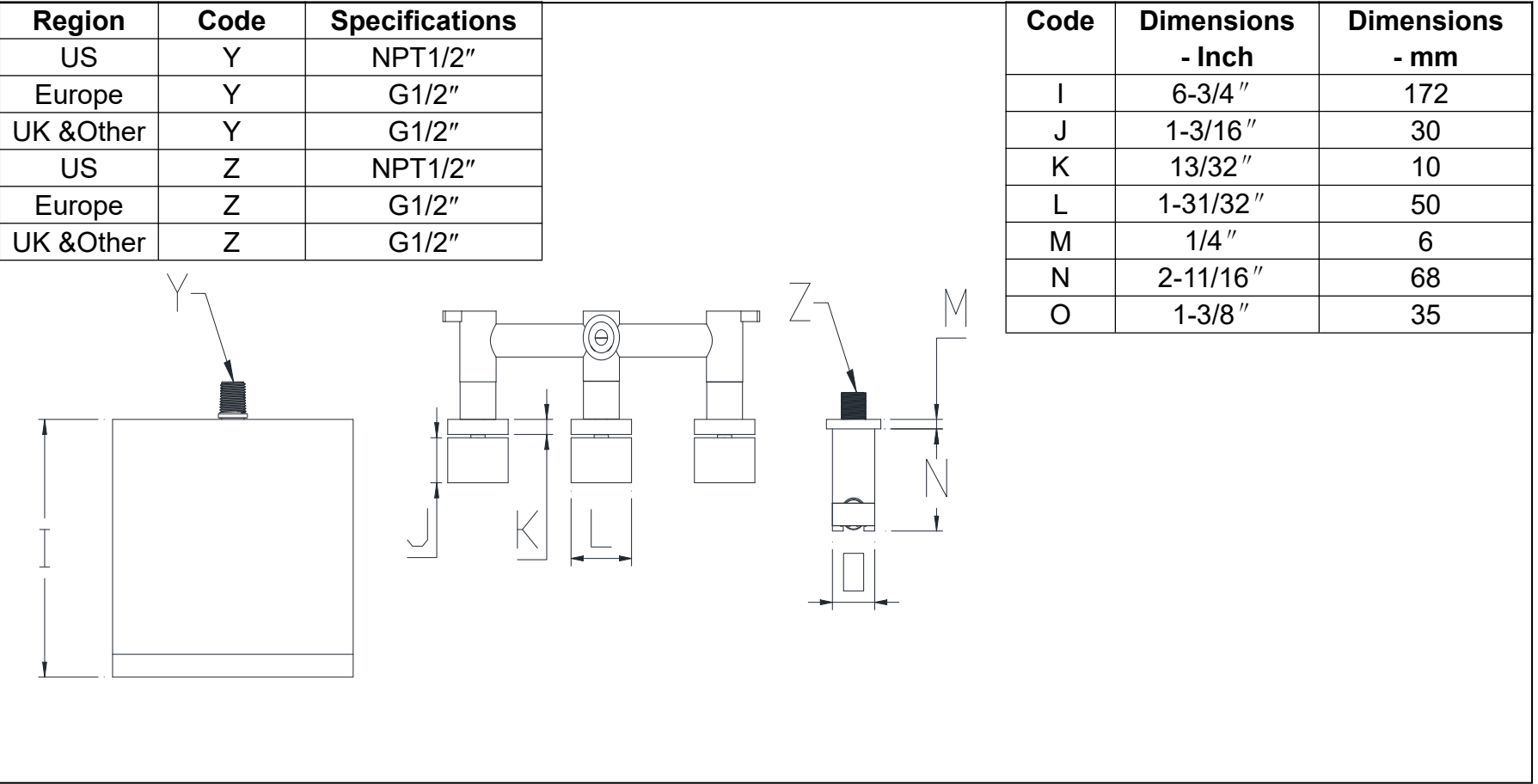
TOP VIEW OF FAUCET
