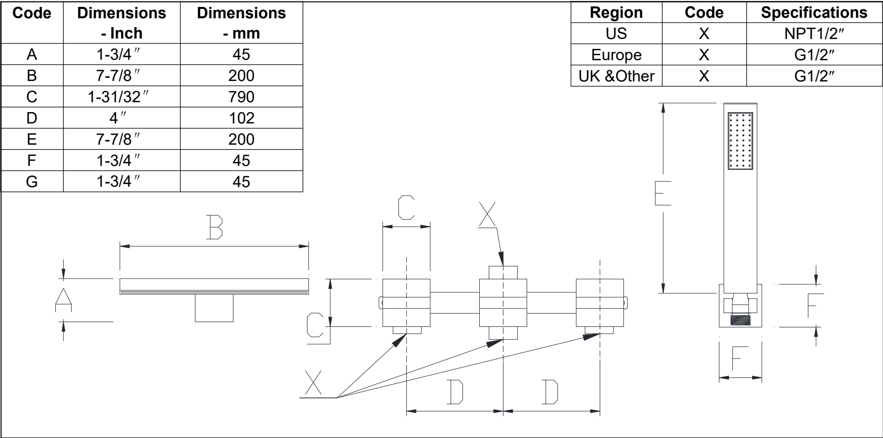
FRONT VIEW OF FAUCET
