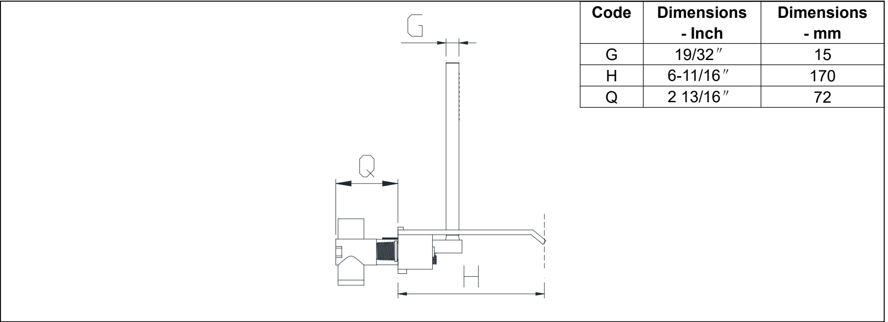
LEFT VIEW OF FAUCET
