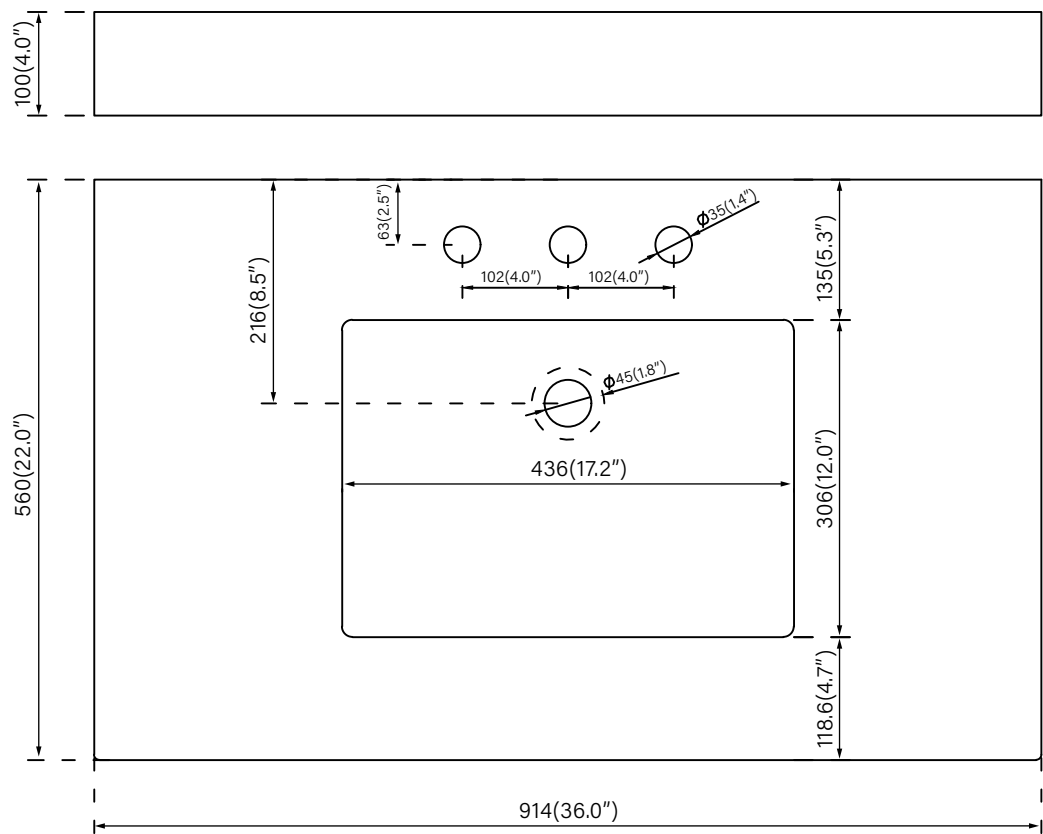
VanityTop
