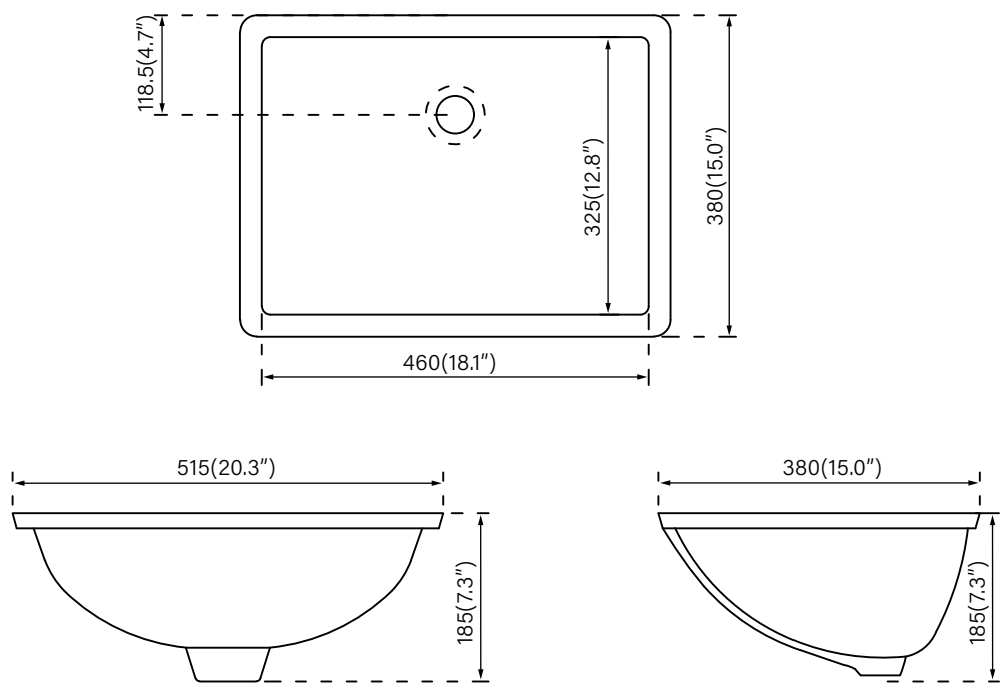
Undermount Sink
