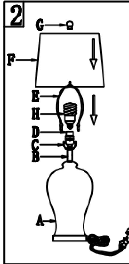
Step2 Insert the Harp (E) into the Saddle (C). Put the shade(F) on the Harp(E),then tighten the Finial (G)into the Harp (E) Insert the bulb(H) into the socket(D).
