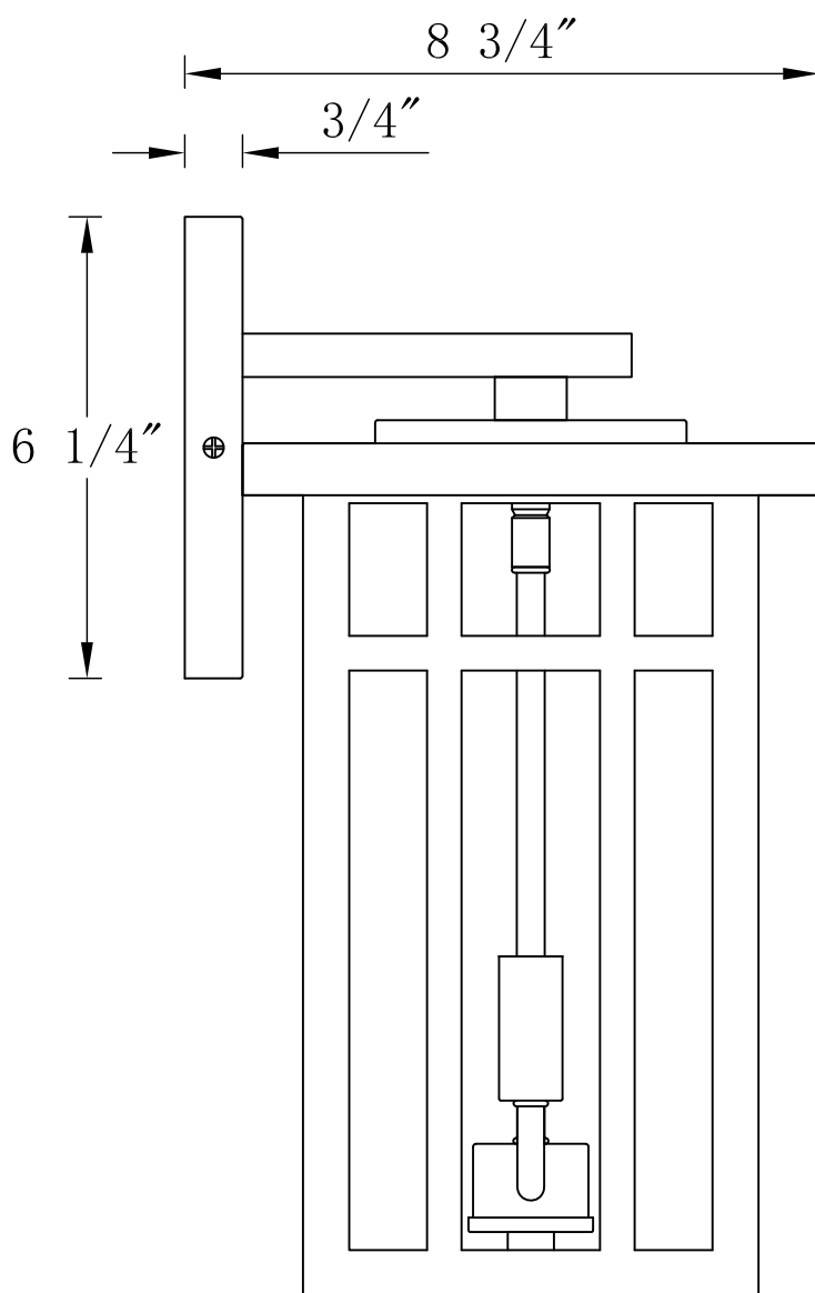
SIDE VIEW
