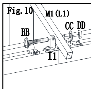
Fig.10: Fix long middle beam(L1) and short middle beam(M1) to middle beam connector(I1), by using bolt (BB)、 flat washer (CC) and nut (DD) .
