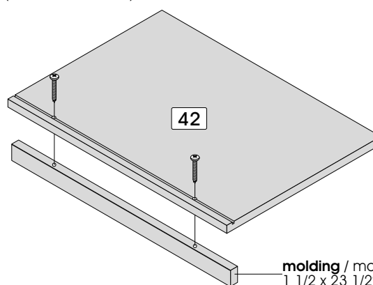
molding / moulure / moldura 1 1/2 x 23 1/2" (38 mm x 597 mm)
