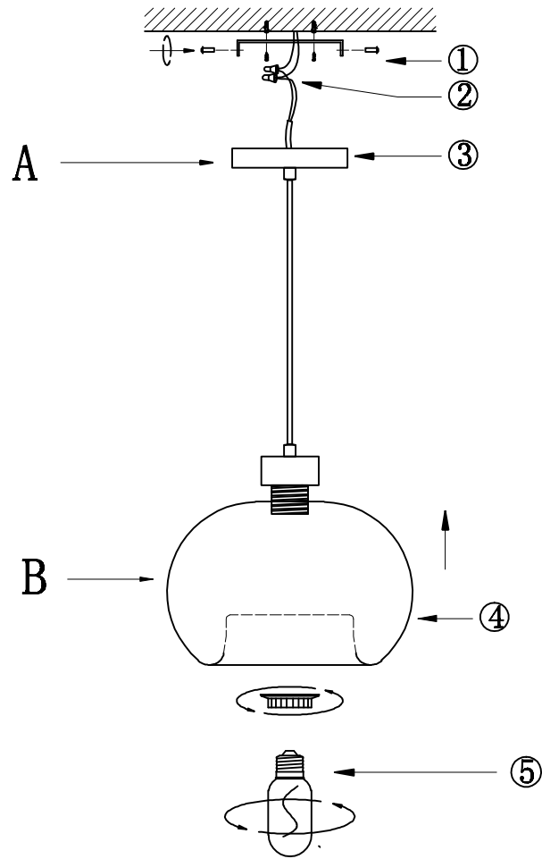
Installation sequence diagram
