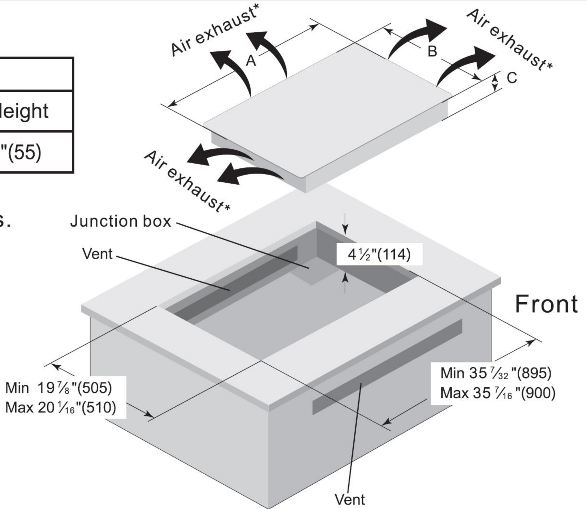
EMPV-IDC36 Cooktop and Cutout Dimension
